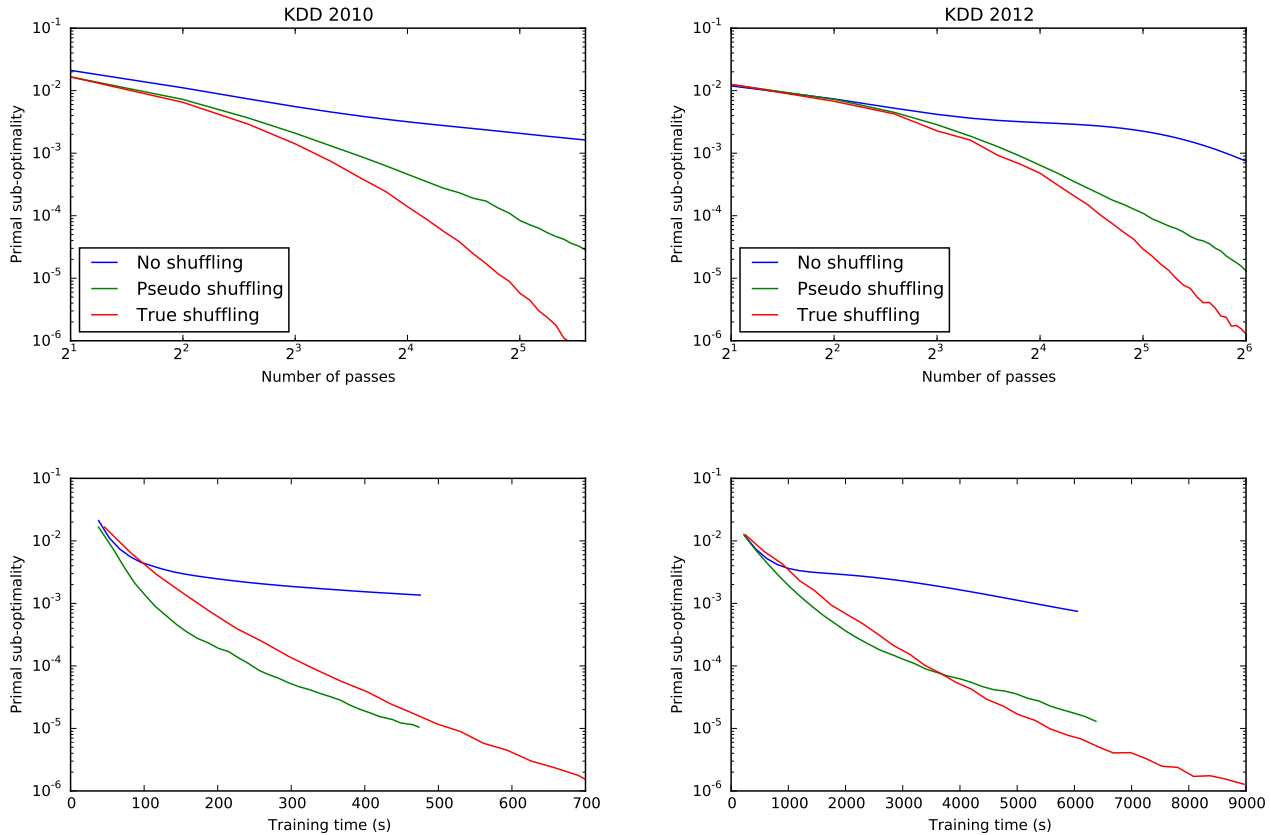
Figure 4: Convergence of SDCA for different shuffling options.
