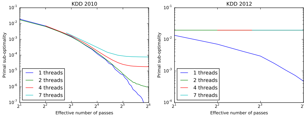
Figure 2: Performance of A-SDCA on two different datasets. Left: KDD 2010 data. Right: KDD 2012 data. The datasets are summarized in Table 1. Log-log scale is used to illustrate the super-polynomial convergence of sequential SDCA.
