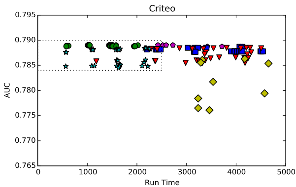
Figure 5: Comparison results. Left: Total run time (in seconds) and AUC of top 20 candidates from each learner. Right: larger display of the dotted region in the left plots. Top: results on KDD 2010 data. Middle: results on KDD 2012 data. Bottom: results on CRITEO data.
