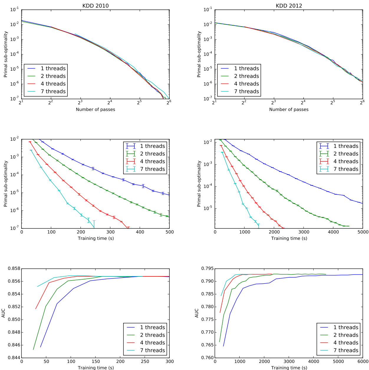
Figure 3: Convergence of SA-SDCA for different number of threads. Left: results on KDD 2010 data. Right: results on KDD 2012 data. Top and middle: primal sub-optimality vs. effective number of passes and training-time, bottom: area under ROC curve for holdout set. Log-log scale for top plots illustrates the super-polynomial convergence rate of the SA-SDCA
